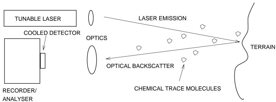
FIG.3.1 SIMPLIFIED SCHEMATIC OF AN LIDAR (ABSORPTION) SPECTROMETER
