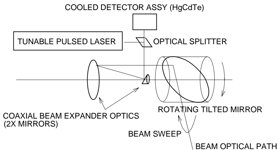
FIG.4 SIMPLIFIED SCHEMATIC OF A LIDAR SPECTROMETER HEAD (RECCE SENSOR)
