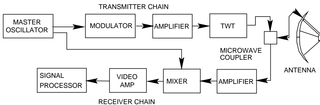
FIG.3.2 GROUNDMAPIING RADAR - FUNCTIONAL MODEL
