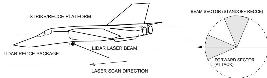
FIG 7.2. CIRCULAR (PPI) SCAN PATTERN AIRBORNE LIDAR ARRANGEMENT
