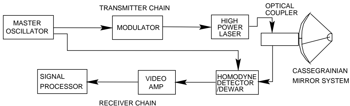
FIG.3.3 SPECTROMETER LIDAR - FUNCTIONAL MODEL
